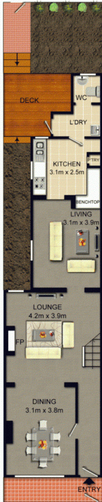
GROUND FLOOR
